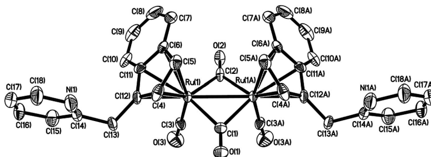
Figure 5. ORTEP diagram of 17 . Selected bond lengths [Å]: Ru(1)–Ru(1A) 2.7389(15).
