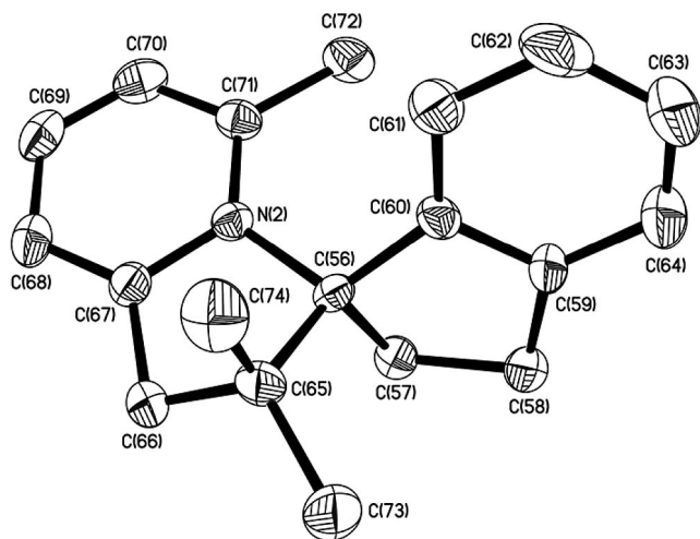
Figure 8. Structure of the cation of 22 .
