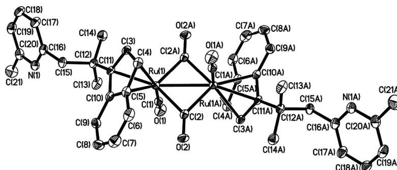
Figure 2. ORTEP diagram of 9 . Selected bond lengths [Å]: Ru(1)–Ru(1A) 2.7443(13).
