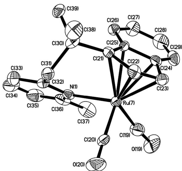
Figure 7. Structure of the cation of 21 .
