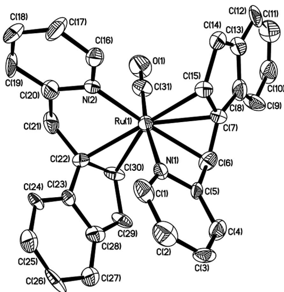
Figure 9. Structure of the cation of 24 .
