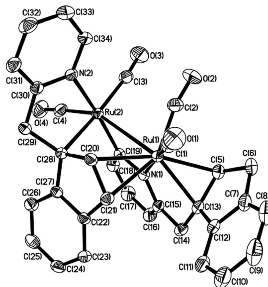
Figure 6. Molecular structure of 18 . Selected bond lengths [Å]: Ru(1)–Ru(2) 2.9448(5), Ru(1)–N(1) 2.088(2), Ru(1)–C(5) 2.228(3), Ru(1)–C(13) 2.256(3), Ru(1)–C(20) 2.371(3), Ru(1)–C(21) 2.323(3), Ru(2)–N(2) 2.188(2), Ru(2)–C(28) 2.211(3), Ru(2)–C(19) 2.044(3), C(5)–C(6) 1.527(5), C(5)–C(13) 1.421(4), C(20)–C(21) 1.414(4), C(20)–C(28) 1.464(4).
